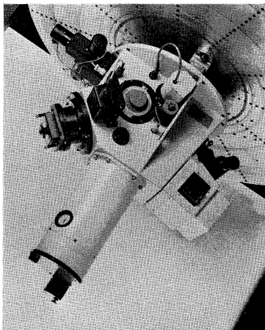
Boller & Chivens Cassegrain Spectrograph
