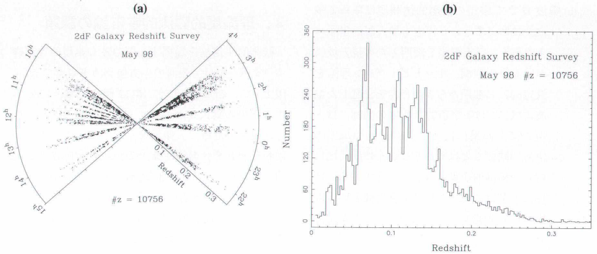
図2 2dF (Two degree Field) 銀河サーベイの現状 13) ：(a) cone diagram, (b) redshift distribution.
