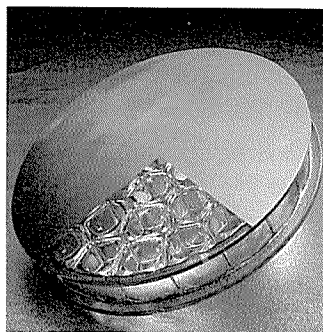
18" diameter, 60% lightweighted mirror blank
