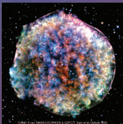
Credit: X-ray: NASA/CXC/RIKEN & GSFC/T. Sato et al., Optical: BSS
